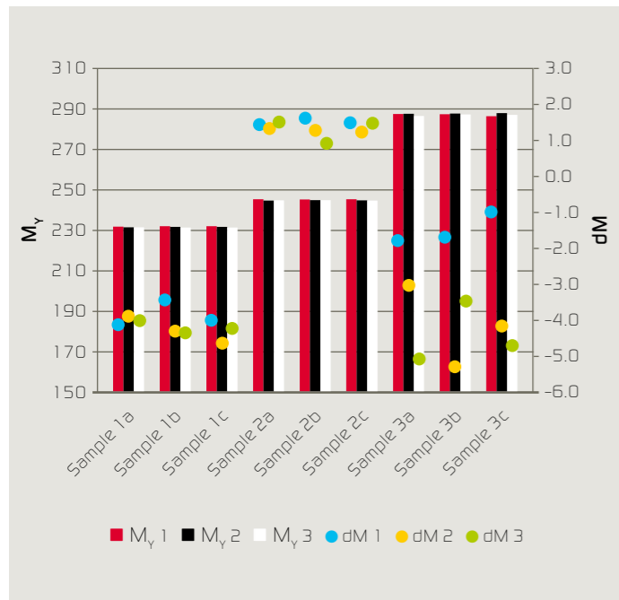
Figure 2: Jetness ( M_V ) and undertone (dM) of samples 1 to 3, measured using the d/8° tabletop instrument at three different spots a, b, c. For each spot, three mean values were determined from five measurements each: M_V and dM 1,2,3.
