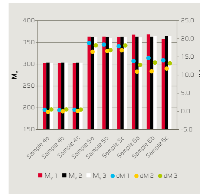
Figure 6: Jetness ( M_V ) and undertone (dM) of samples 4 to 6, measured using the 45°/0° handheld instrument at three different spots a, b, c. For each spot, three mean values were determined from five measurements each: M_V and dM 1,2,3.
