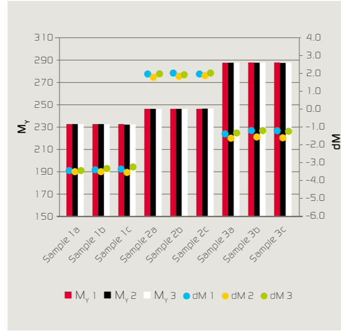
Figure 3: Jetness ( M_V ) and undertone (dM) of samples 1 to 3, measured using the 45°/0° handheld instrument at three different spots a, b, c. For each spot, three mean values were determined from five measurements each: M_V and dM 1,2,3.
