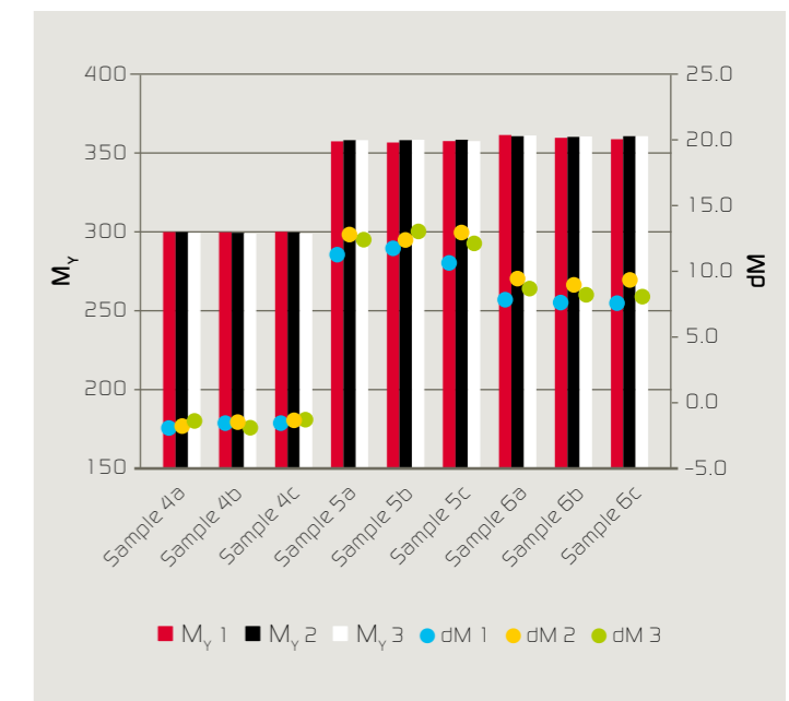
Figure 7: Jetness ( M_V ) and undertone (dM) of samples 4 to 6, measured using the 45°/0° tabletop instrument at three different spots a, b, c. For each spot, three mean values were determined from five measurements each: M_V and dM 1,2,3.
