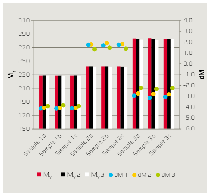
Figure 4: Jetness ( M_V ) and undertone (dM) of samples 1 to 3, measured using the 45°/0° tabletop instrument at three different spots a, b, c. For each spot, three mean values were determined from five measurements each: M_V and dM 1,2,3.
