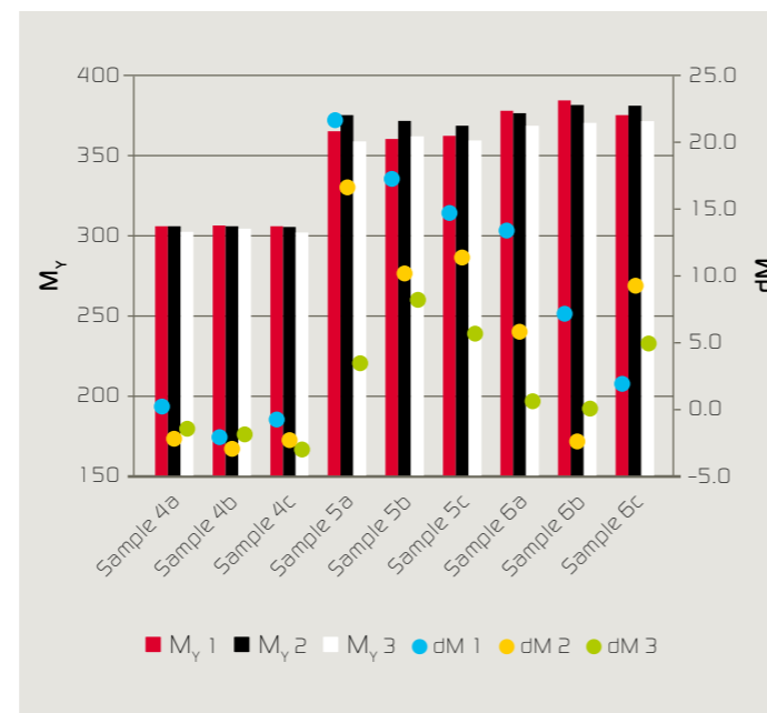
Figure 5: Jetness ( M_V ) and undertone (dM) of samples 4 to 6, measured using the d/8° tabletop instrument at three different spots a, b, c. For each spot, three mean values were determined from five measurements each: M_V and dM 1,2,3.
