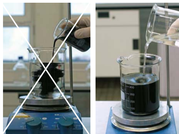
Dilution of the Mill Base to the final Dispersion and/or Inkjet Ink: Improper (left) and correct Process (right) to prevent Dispersion Shock
