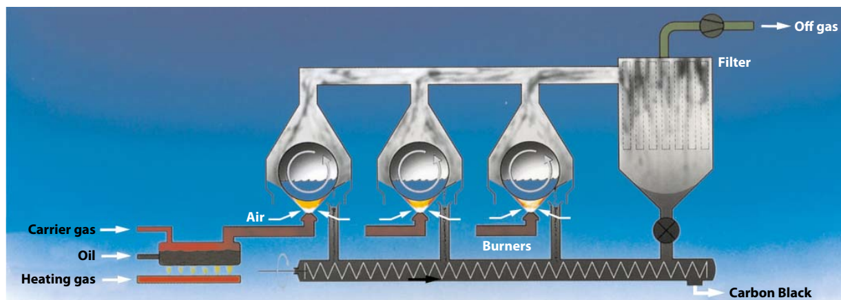
Figure 3 Schematic Depiction of the Degussa Gas Black Process.
