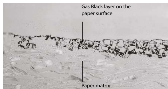
Transmission Electron Microscopic Image (microtome Section) of plain Paper printed with a Gas Black-based Inkjet Ink
