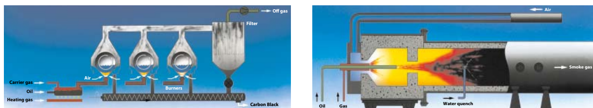
Figure 4 Key Differences between Furnace Blacks and Gas Blacks.
