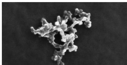
Figure 15: Electron microscope view of gas black particles (COLOUR BLACK FW 285)
