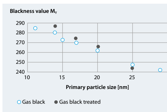
Figure 28: Primary particle size and jetness
